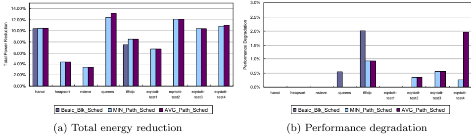
Fig. 6. Simulation results when using the power-gating control for integer and floating-point units ( \text{BreakEven}_C = 32 )
