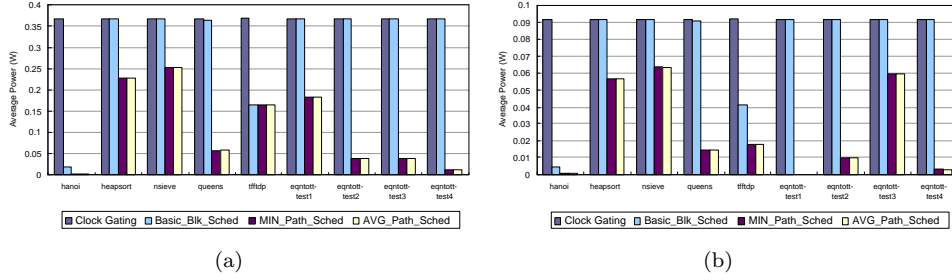
Fig. 5. Power gating on (a) Floating-Point Adder and (b) Floating-Point Multiplier for miscellaneous benchmarks ( \text{BreakEven}_C = 32 )
