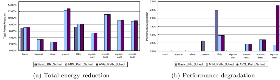
Fig. 8. Simulation results (out-of-order issue) when using the power-gating control for integer and floating-point units ( \text{BreakEven}_C = 32 )
