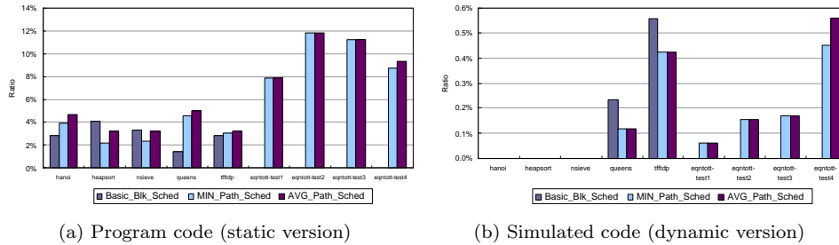
Fig. 7. Ratio of power-gating instructions to total instructions when using the power-gating control for integer and floating-point units ( \text{BreakEven}_C = 32 ).
