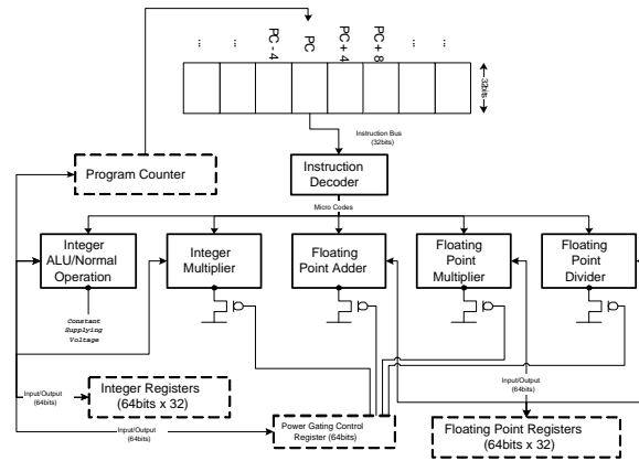
Fig. 1. Machine architecture model with power-gating control
